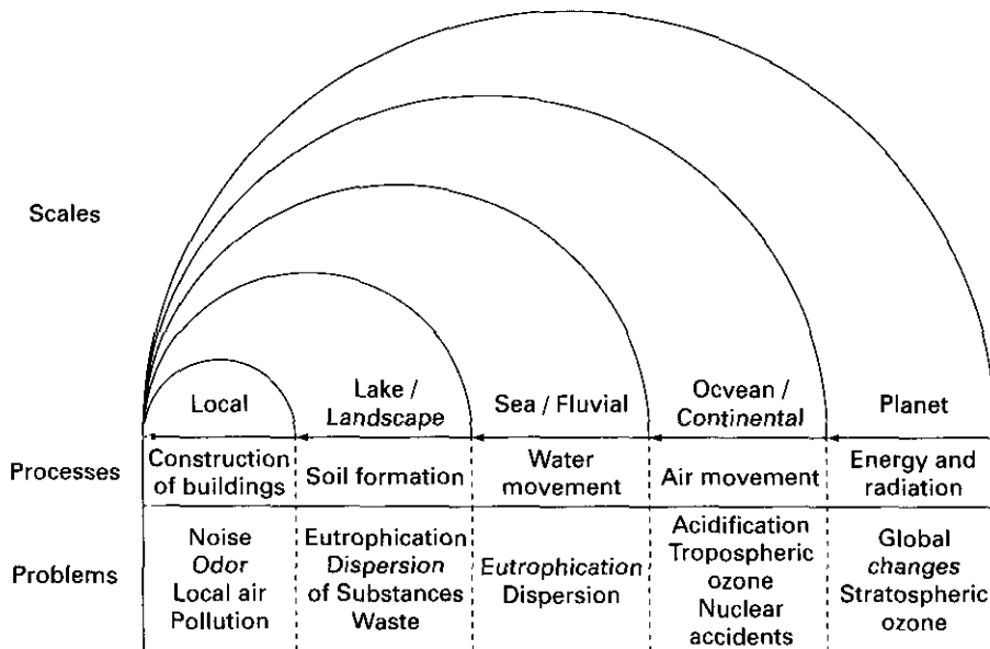
Figure 1. Geographical scales of environmental problems; processes and problems characteristic for local, regional, fluvial, continental and planetary scales.
