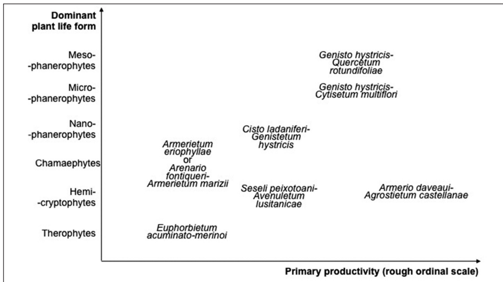
Figure 3. – Diagrammatic representation of the Genisto hystricis-Quercus rotundifoliae Sigmoidetum, the climatophilous vegetation series of the ultramafic rocks of northeastern Portugal.
