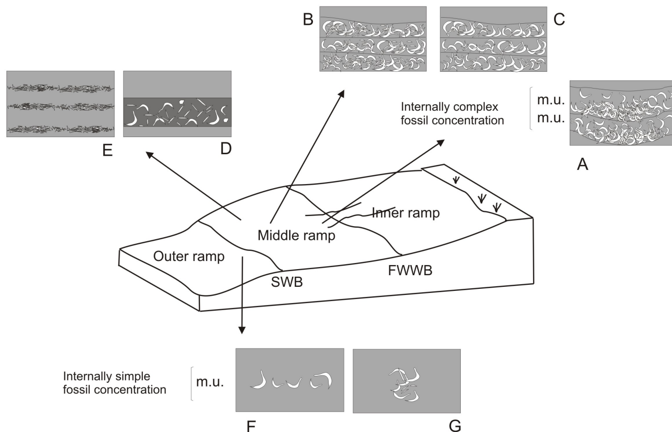
Fig. 5.- Schematic diagram showing the distribution of fossil concentrations in the Unit 1 of La Manga Formation. SWB, storm wave base, FWWB, fair-weather wave base.
