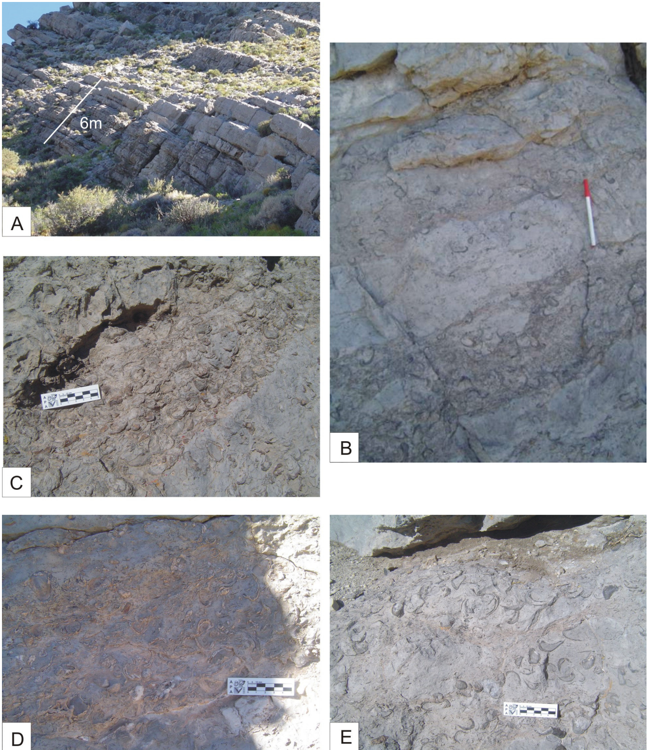
Fig. 3. (This page and the opposite one) A- General aspect of Unit 1 in Barda 2; B- Detail of coarsening upward cycles. Note the pack-stone-grainstone centimetric intervals (bioclastic concentrations of type B ) (pen for scale 15 cm); C to K- Fossil concentrations of La Manga Formation: C- Type A , channelized fossil concentrations of Gryphaea sp.; D- Type B , shell beds of Gryphaea sp. highly reworked; E- Type C , shell beds of Gryphaea sp. moderately reworked; F- Type D , fossil concentrations of Gryphaea sp. with biomicritic to biopelmicritic matrix; G- Type E , shell detritus (pen cap for scale is 4 cm); H- Type F , accumulations of echinoderm spines produced by bottom currents in a top surface view; I- Type F , fossil concentrations produced by bottom currents (in cross section). Note the presence of corals and gryphaeid levels; J- Shell concentrations of Type G in clumps; K- Association of bioclastic concentrations types E and F .
