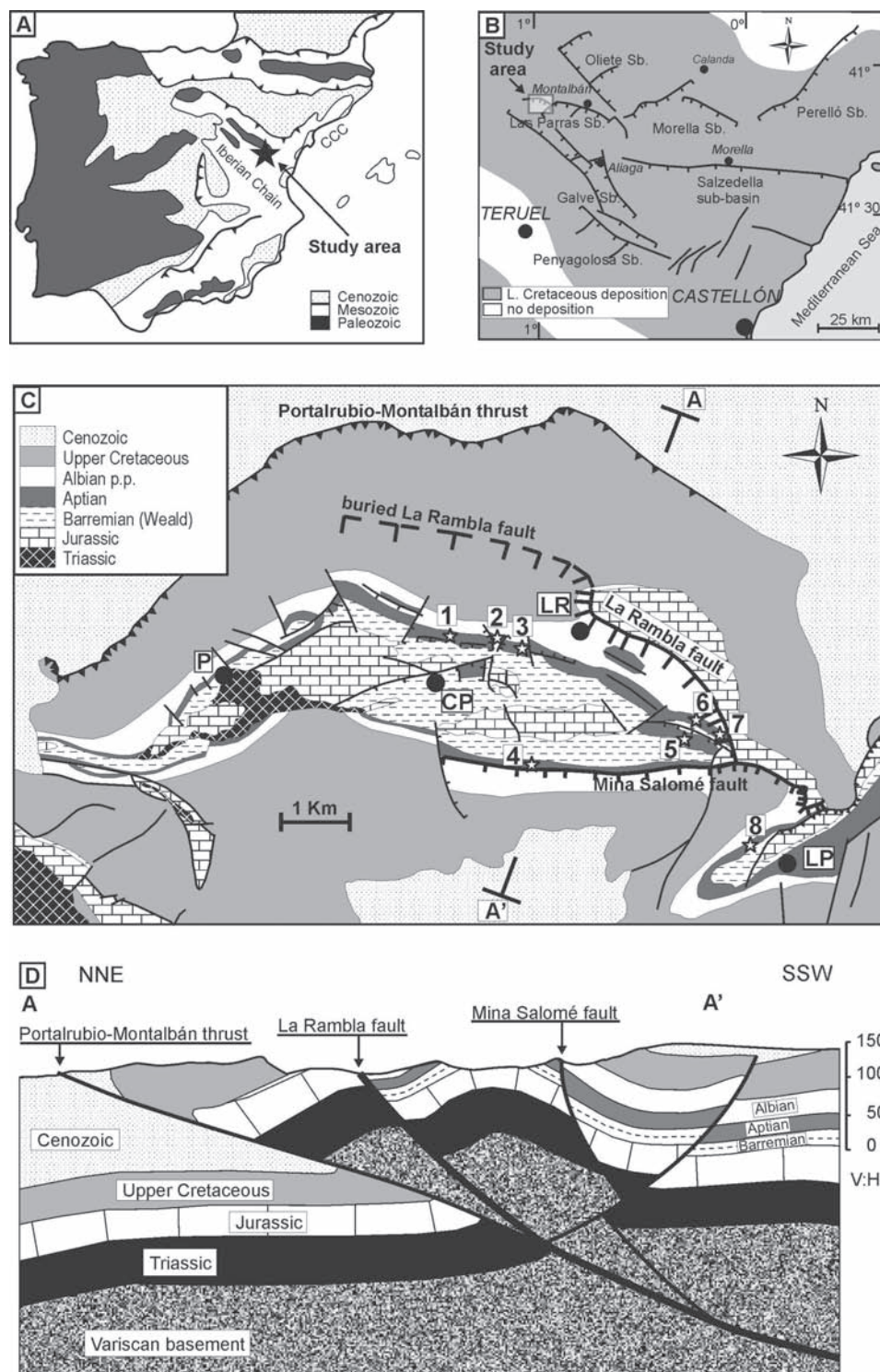
Fig. 1.- A) Geographic and geological context of the studied area. CCC Catalanian Coastal Chain. B) Main structural features of the Maestrazgo basin and sub-basins (Sb) during the lower Cretaceous. Modified after Liesa et al. (2004). C) Geological map of the studied area. Modified after Martín Fernández (1979) and Soria (1997). Localities: P, Portalrubio; CP, Cuevas de Portalrubio; LR, La Rambla de Martín; LP, Las Parras del Martín. Numbers 1 to 8 correspond to measured sections. D) Geological cross section representative of the studied area. Without vertical exaggeration. Location is indicated in Fig. 1C. Modified after Liesa et al. (2000).
