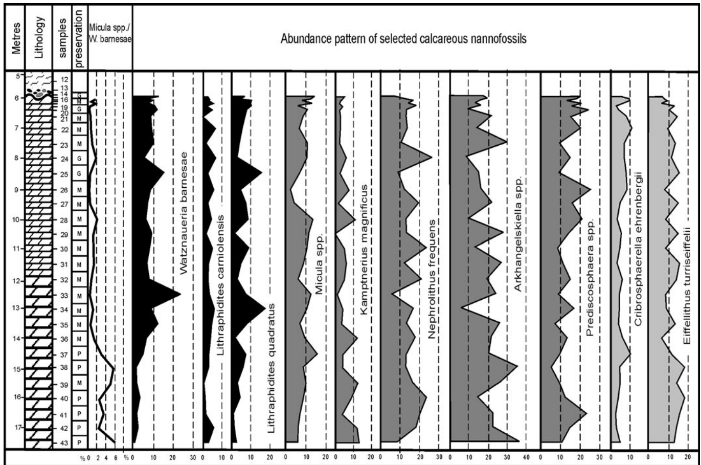
Fig. 8.- Quantitative analysis of calcareous nannofossil distribution in the Maastrichtian, Klyuchi 1 section.
