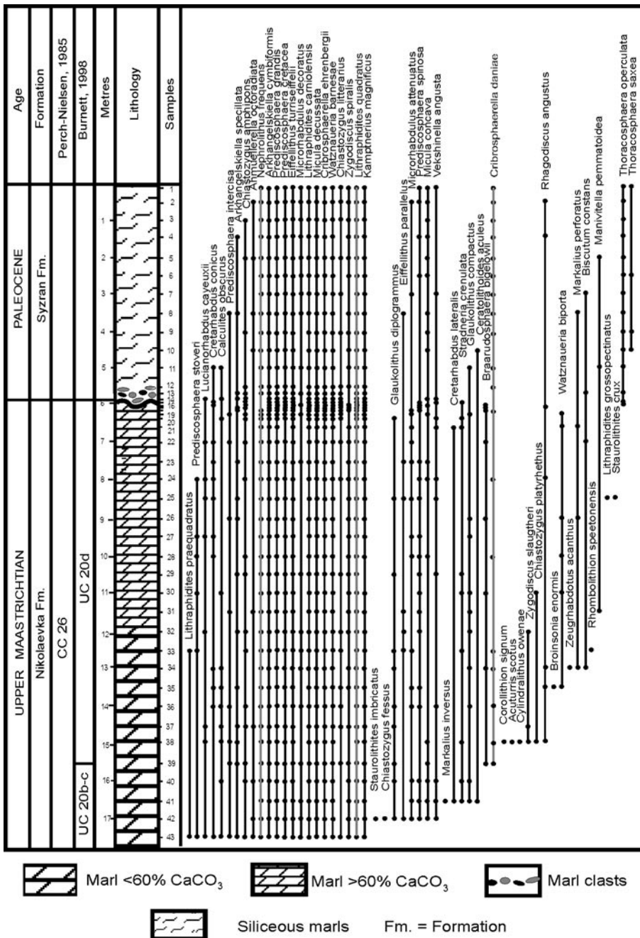
Fig. 5.- Stratigraphic distribution of calcareous nannofossils in the Maastrichtian, Klyuchi 1 section.
