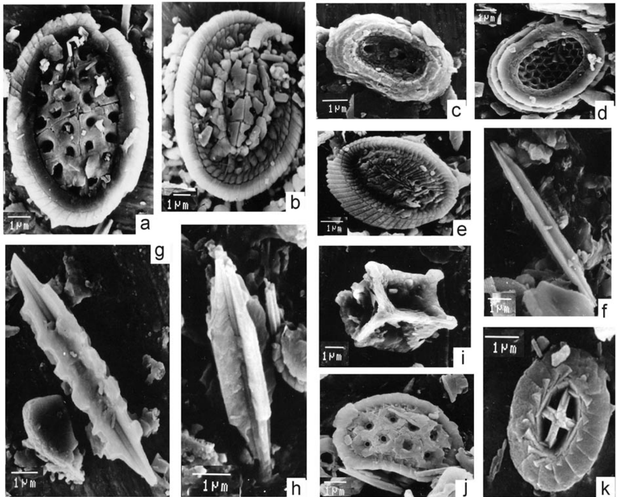
Fig. 10.- (a) Arkhangelskiella specillata Vekshina, Upper Maastrichtian, sample K12-23. Scale bar 1 µm. (b) Broinsonia parca constricta Hattner et al. , Lower Maastrichtian, sample Lkh-15. Scale bar 1 µm. (c) Cribrosphaerella daniae? Perch-Nielsen, Upper Maastrichtian, sample K11-34. Scale bar 1 µm. (d) Cribrosphaerella ehrenbergii (Arkhangelsky) Deflandre, Upper Maastrichtian, sample K11-36. Scale bar 1 µm. (e) Kamptnerius magnificus Deflandre, Upper Maastrichtian, sample K12-24. Scale bar 1 µm. (f) Lithraphidites carniolensis Deflandre, Upper Maastrichtian, sample Lkh 53. Scale bar 1 µm. (g) Lithraphidites grossopectinatus Bukry, Upper Maastrichtian, sample K11-33. Scale bar 1 µm. (h) Lithraphidites quadratus Bramlette and Martini, Upper Maastrichtian, sample K12-16. Scale bar 1 µm. (i) Micula decussata Vekshina, Upper Maastrichtian, sample TP2-28. Scale bar 1 µm. (j) Nephrolithus frequens Gorka, Upper Maastrichtian, sample K12-20. Scale bar 1 µm. (k) Prediscosphaera stoveri (Perch-Nielsen) Shafik and Stradner, Upper Maastrichtian, sample TP2-18. Scale bar 1 µm.
