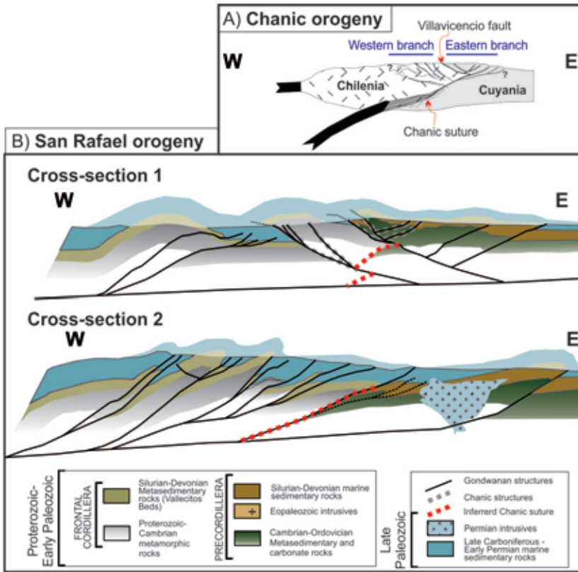
Fig. 5.- A) Conceptual model for the tectonic context of the Chanic orogeny, based on the reconstruction of the Gondwanan deformation along cross-section 1 (Fig. 3). B) Reconstruction of the Gondwanan late Carboniferous-Early Permian fold-and-thrust belt by back stripping the base of the Permo-Triassic volcanics and Triassic rift-related sediments to their horizontal depositional line, using in the cross sections shown in Fig. 3. Cross-section 1 suggests the existence of a dual vergence thrust system, probably influenced by the Late-Devonian-early Carboniferous (Chanic) structural grain. In cross-section 2, the Proto-Frontal Cordillera has a predominantly eastward vergence in the Gondwanan structures, with an incipient development of a Proto-Precordillera.
