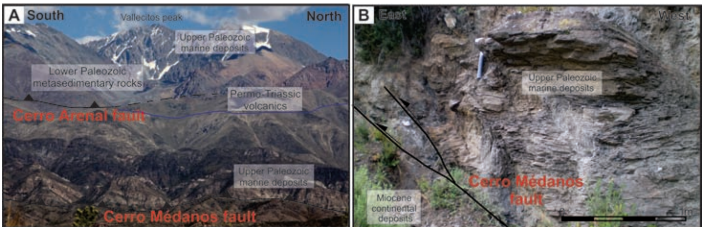
Fig. 6.- A) Photograph looking west of the main Andine structures of the La Carrera fault system, eastern slope of the Cordón del Plata range. B) Detailed of the Cerro Médanos fault uplifting marine sedimentary rocks of the upper Carboniferous (El Plata Formation) on top of the Miocene synorogenic units.
