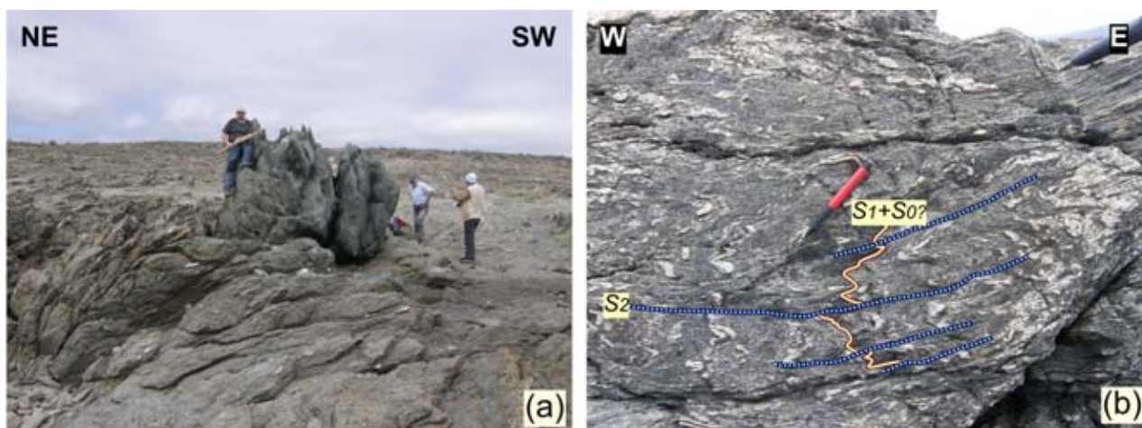
Fig. 9.- Photographs of the (a) boudin in the metabasites of the ChMC in El Peñón area, and (b) D2 recumbent folds in the Punta Claditas zone. Location at coordinates (a) 31° 31' 47" S, 71° 34' 23" W; (b) 31° 31' 17" S, 71° 34' 31" W.
