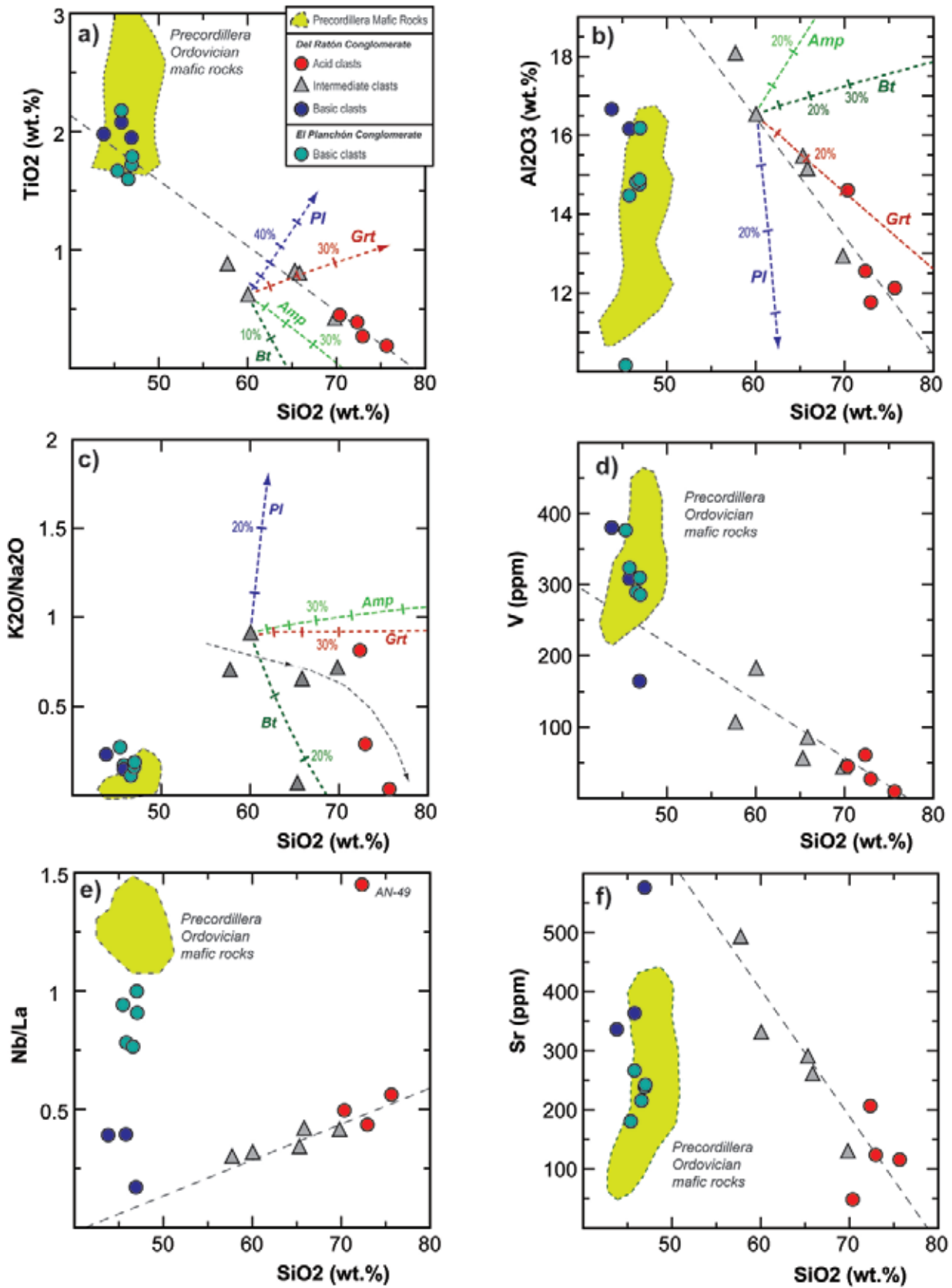
Fig. 8.- Diagrams of SiO 2 vs. major and trace elements (TiO 2 , Al 2 O 3 , V, Sr) and element ratios (K 2 O/Na 2 O, Nb/La). Black dashed line shows the approximate trend defined by part of the rocks plotted. Basic rocks fall away from these trends defined by the acid-intermediate compositions. Colour dashed lines are linear mixing models generated by the fractionation of different mineral phases from a selected starting composition (Del Ratón Formation sample AN22). Marks on the lines are intervals of 10% crystallization.
