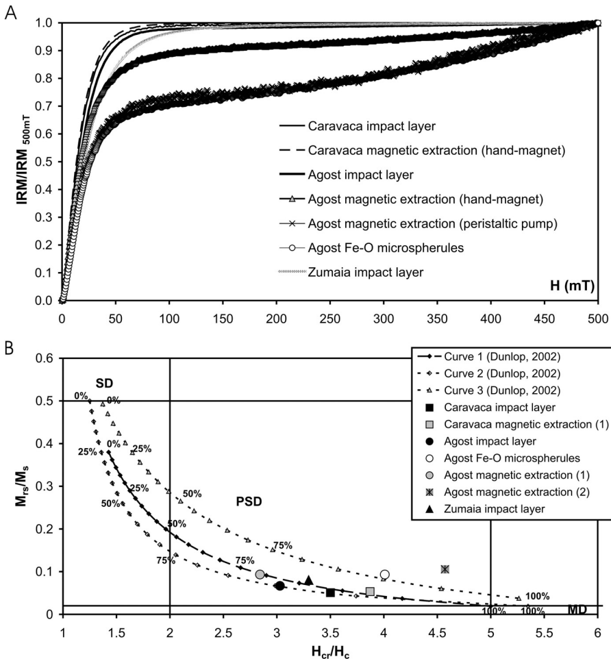
Figure 18. A) IRM back-demagnetization curves (rescaled and normalized) for impact layer samples, microspherules and magnetic extractions (Caravaca, Agost and Zumaya). B) Dayplot for impact layer samples, Fe-O microspherules and magnetic extractions; curves 1, 2 and 3 (Dunlop, 2002 a, b) correspond to mixtures of different SD and MD end-members, with % indicating the fraction of MD material in each case; boundaries for SD, PSD and MD regions are from Dunlop (2002 a, b).
