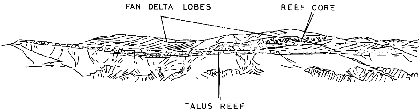
Fig. 13.—Panoramic view of reefs adapted to fan-delta lobes in Canteras hill.
