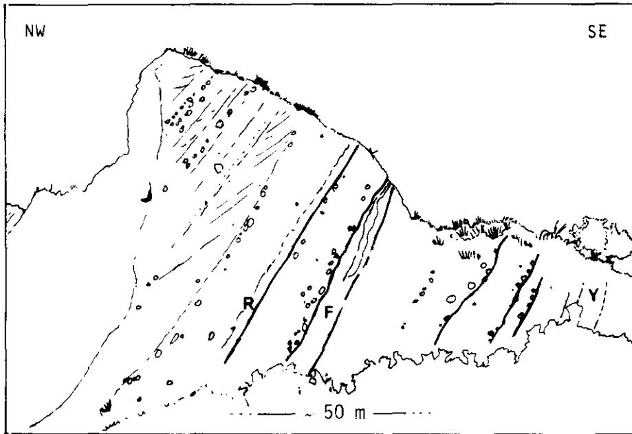
Fig. 26.—Panorama of STOP 3 - 1 A with the Segura Conglomerates exposed in a quarry behind the lemon trees which partly block the view of the lower part. Note two olive trees standing to the right for approximate scale. Same letters as in figures 27 and 28. Top of the section to the north (left of the observer).
