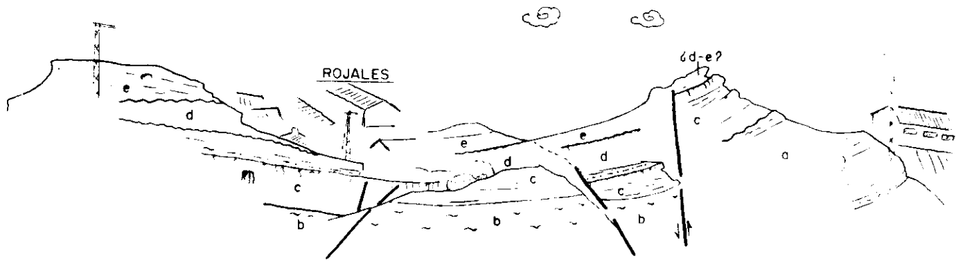
Fig. 30.—Outcrop of the Plio-Pleistocene continental and marine deposits in Rojasles (Lower Segura Basin). a, b, c, d, e: are Units described in figure 31 (After Goy et al. , 1990).
