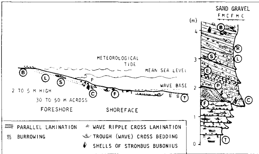
Fig. 39.—(A) Typical beach profile for Mediterranean gravelly coasts. (B) Composite sequence of facies generated by progradation of gravelly beaches. Key: B: berm; R: ridge and runnel system; L: parallel lamination; S: ephemeral, secondary berms; E: erosional surfaces; P: plunge step at the base of the foreshore; C: coarse pebbles and boulders (P & C: indicate the breakers zone); F: fining upward sequences; T: transition zone (Modified after Dabrio et al. , 1985).
