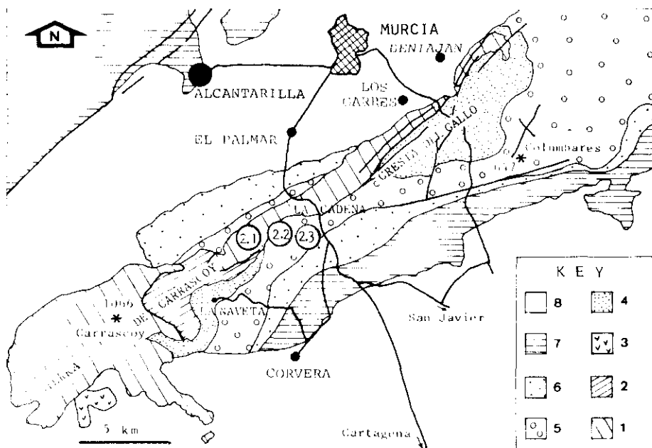
Fig. 14.—Schematic geological map of Sierra de Carrascoy (Murcia). Legend: (1): Alpujárride (grey phyllades) and Ballabona - Cucharón (red mudstones, limestones and dolostones) Complexes; (2): Maláguide Complex (red mudstones and quartzites, followed upwards by dark grey dolostones) (1 & 2, Betic substratum); (3): Volcanic rocks; (4): conglomerates and turbidites (Tortonian I); (5): «Puerto de la Cadena conglomerates» (fan deltas, Tortonian II to Messinian I); (6): basinal marls and turbidites («Torremendo marls») and La Virgen calcarenites (Tortonian II to Messinian I); (7): Mio - Pliocene marls and conglomerates (8): Plio - Quaternary rocks. Encircled: location of STOPS 2-1, 2-2 and 2-3.
