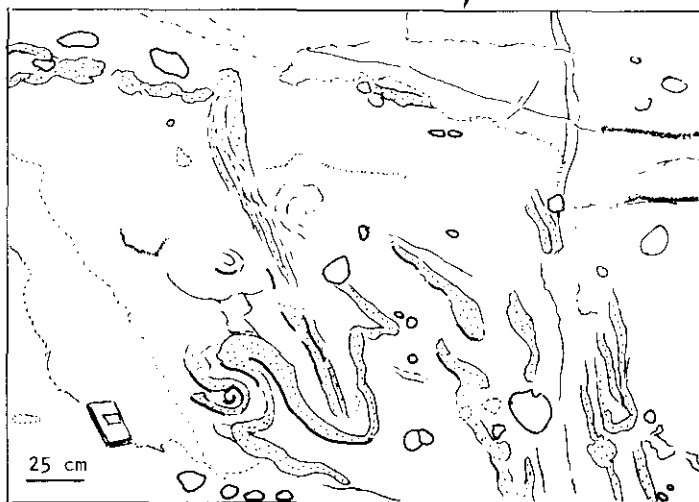
Fig. 18.—Above: a fossiliferous layer of yellow sandstones with scattered pebbles and water-escape deformation at the top of a transgressive sequence of fan-delta lobe. Note a thicker layer of conglomerates (facies C-2, see Table I) behind people standing on the road. Below: detail of deformation; dotted layers are more cemented sandstone layers.
