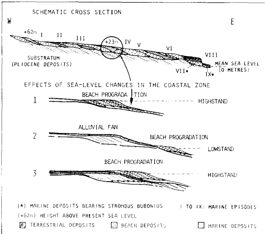
Fig. 35.—Development of an offlapping sequence of coastal and terrestrial units caused by relative changes of sea level in the Cope Basin (modified after Bardají et al. , 1987 and Goy et al. , 1989 a).
