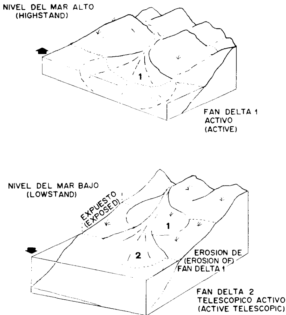
Fig. 36.—Sedimentary processes and development of fan-delta units in response to relative changes of sea level in Cope Basin (after Goy et al. , 1989 a).
