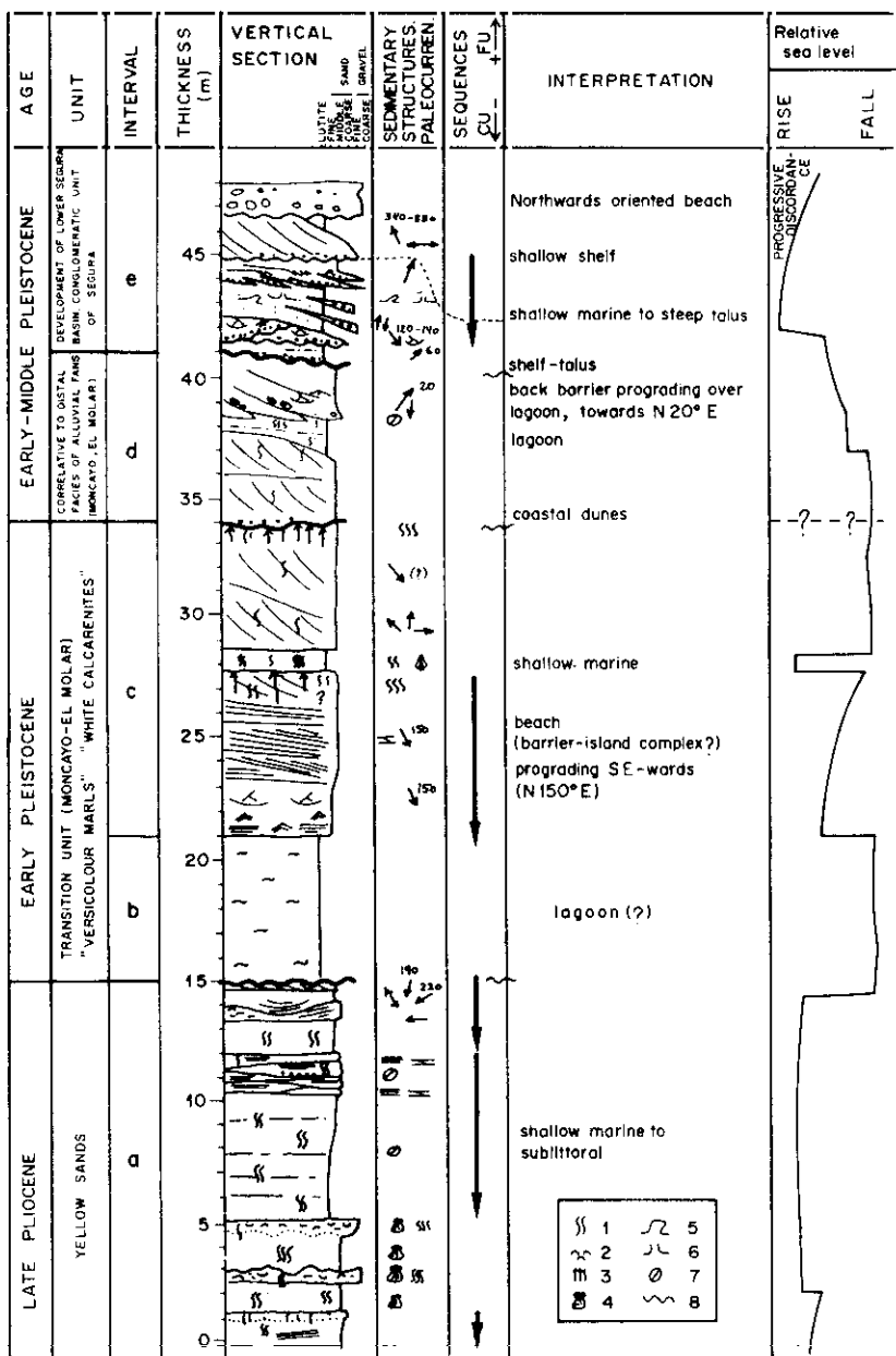
Fig. 31.—Section of Rojas. Sequence of Plio-Pleistocene marine and terrestrial deposits (after Goy et al. , 1990).
