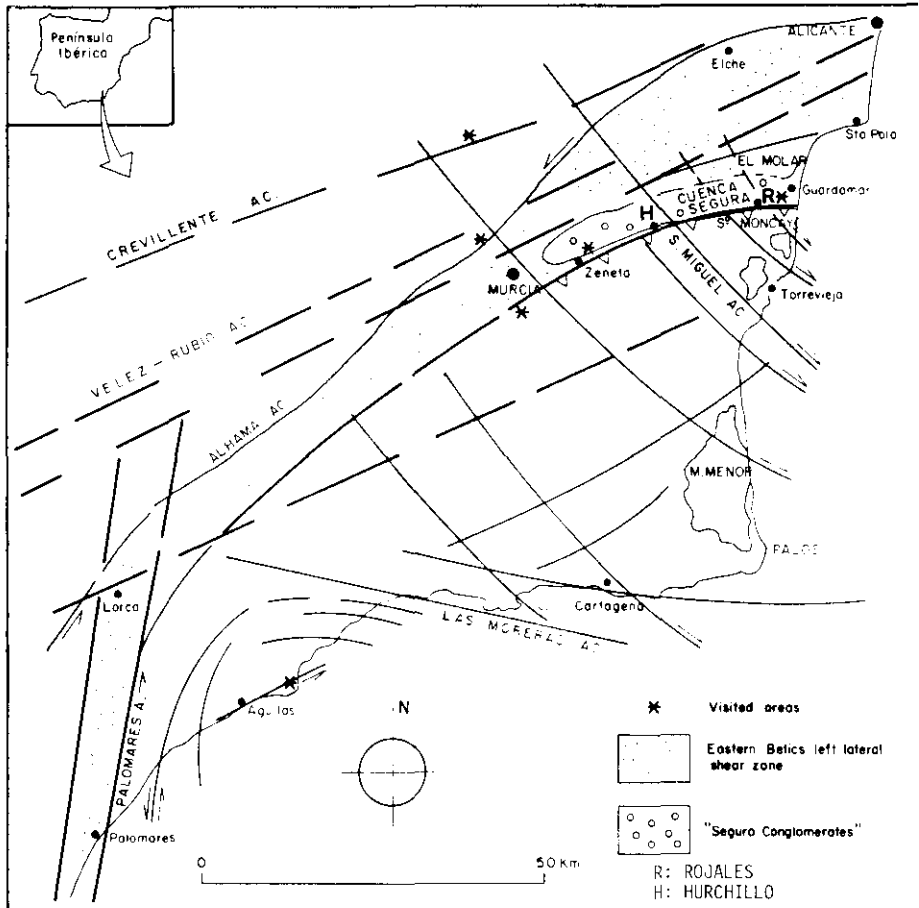
Fig. 3.—Location map of the area visited during the workshop inside the «left lateral shear zone» and main tectonic structures active during Quaternary (modified after Boccaletti et al. , 1987; Montenat et al. , 1987; Goy & Zazo, 1989 and Somoza, 1989).
