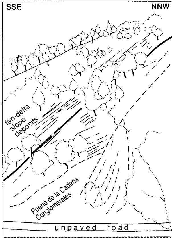
Fig 3.—Sketch drawn from a photograph of the unconformable limit (thick line) between the studied deposits and the Puerto de la Cadena conglomerates near the Casa Motor and La Naveta farm, ca. 250 m WSW from km 403.3 (national road 301). Modified and re-interpreted from Dabrio et al. 's (1991) figure 20.
