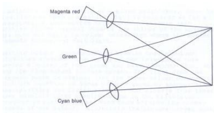
Schematic representation of an additive colour process. By way of three coloured light sources (blue, green and red) three black-and-white transparencies produced from the corresponding red, green and blue separations, are projected in superimposition.
